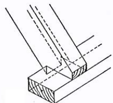
SHOULDERED TOE JOINT
