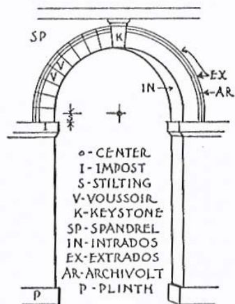
ROUND ARCH, STILTED
