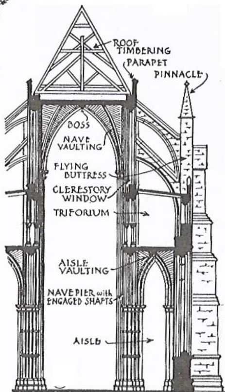
GOTHIC CATHEDRAL TRANSVERSE SECTION (SOUTH SIDE, WESTMINSTER)
