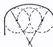
3-CENTERED
