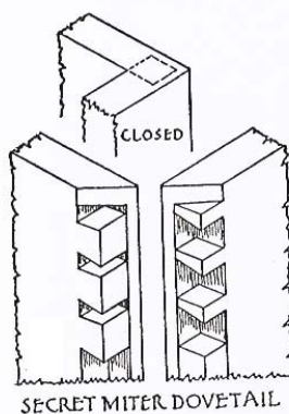
SECRET MITER DOVETAIL
