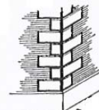
STONE QUOINS IN BRICKWORK
