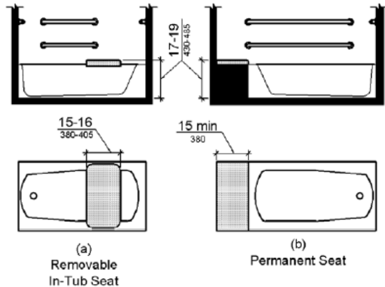
Figure 610.2 Bathtub Seats
