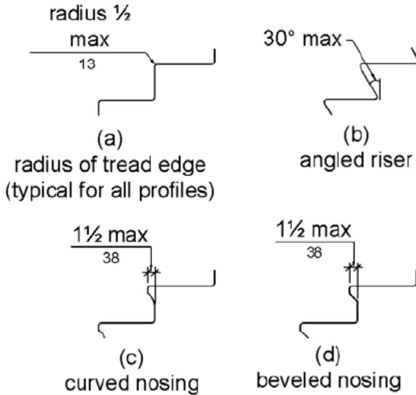
Figure 504.5 Stair Nosings
