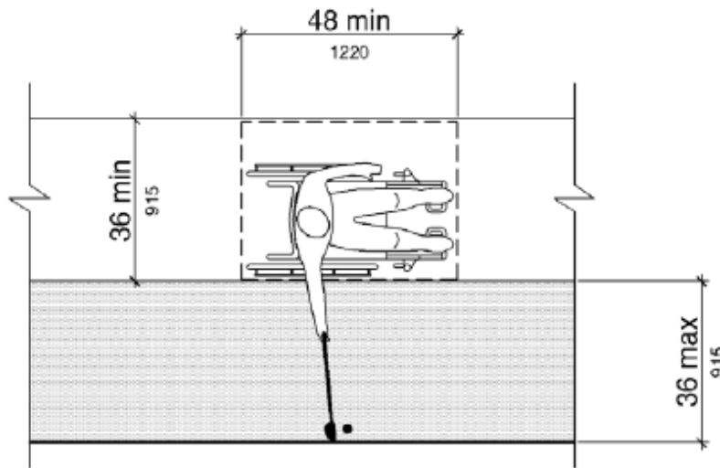
Figure 1007.3.2 Golf Club Reach Range Area
