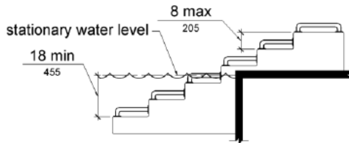
Figure 1009.5.4 Transfer Steps
