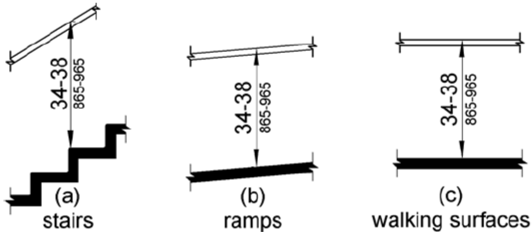
Figure 505.4 Handrail Height
