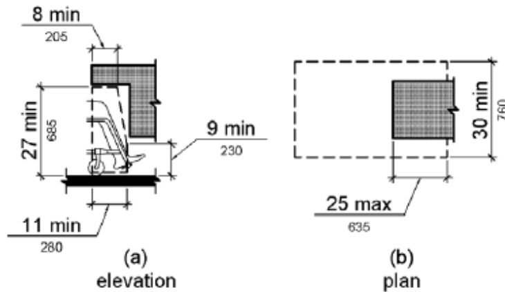
Figure 306.3 Knee Clearance
