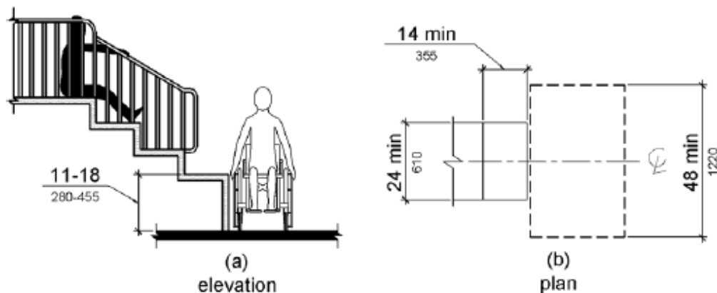
Figure 1008.3.1 Transfer Platforms
