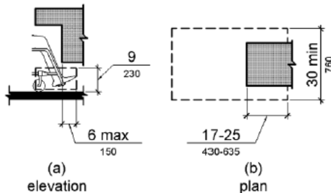
Figure 306.2 Toe Clearance
