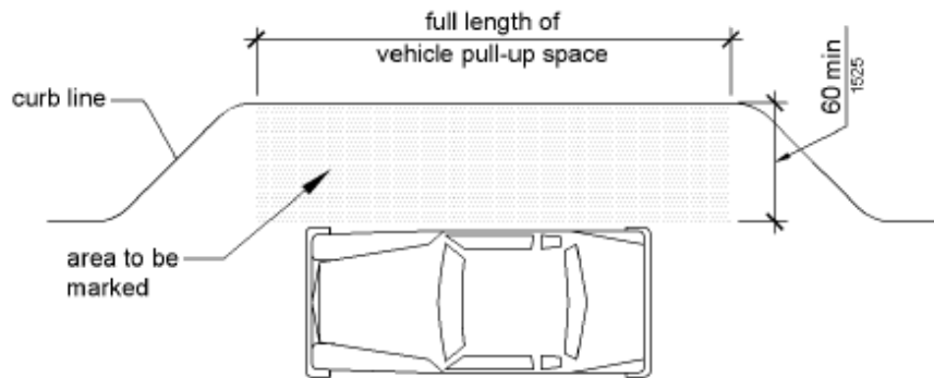
Figure 503.3 Passenger Loading Zone Access Aisle
