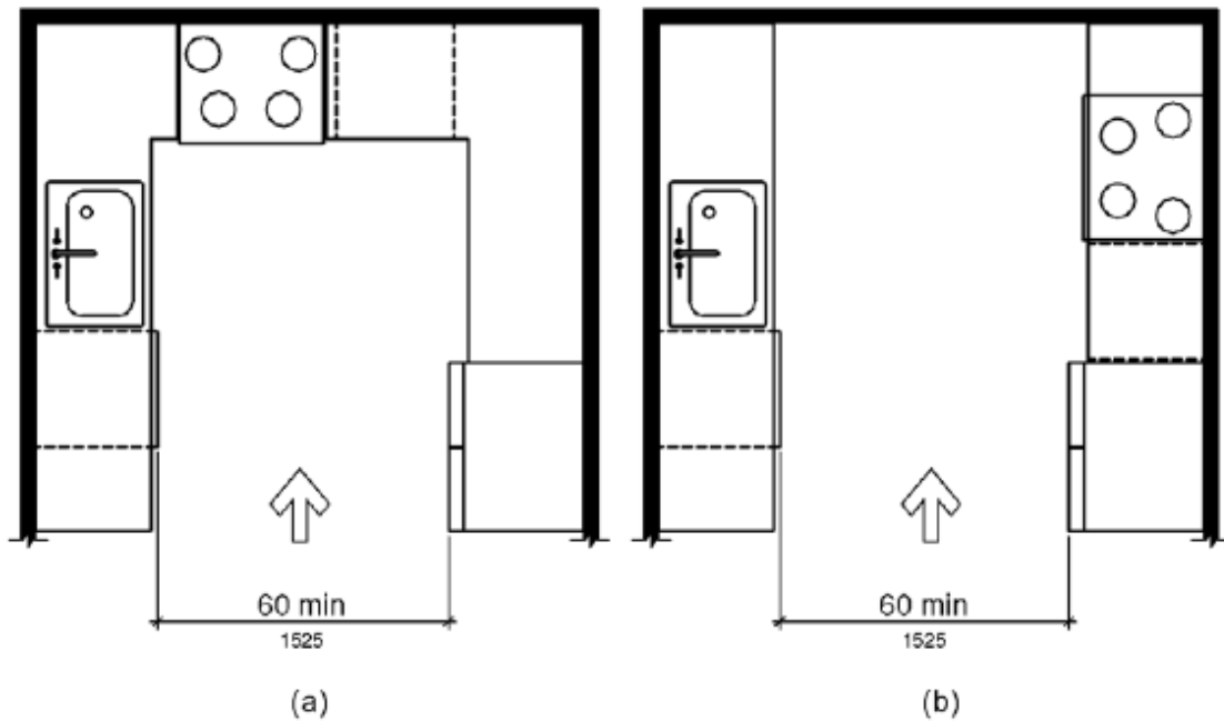
Figure 804.2.2 U-Shaped Kitchens
