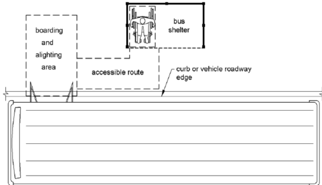
Figure 810.3 Bus Shelters
