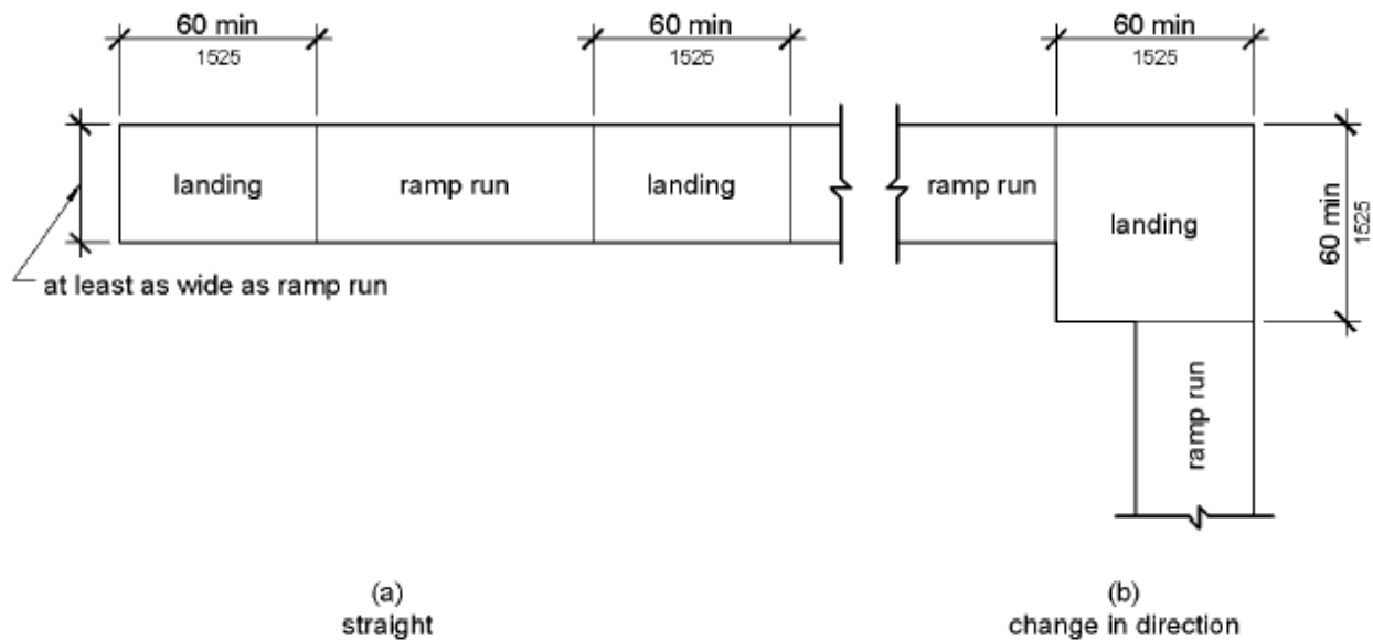
Figure 405.7 Ramp Landings
