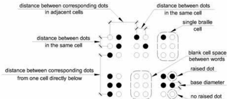
Figure 703.3.1 Braille Measurement
