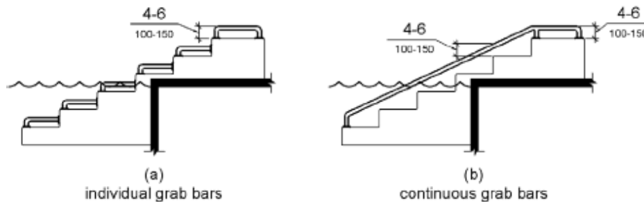
Figure 1009.5.7 Grab Bars
