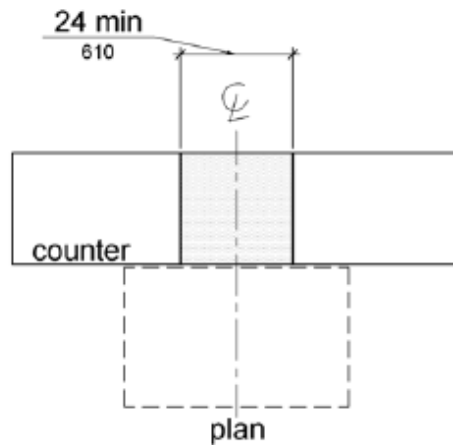
Figure 904.4 (Exception) Alteration of Sales and Service Counters
