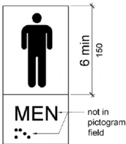
Figure 703.6.1 Pictogram Field
