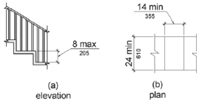
Figure 1008.3.2 Transfer Steps
