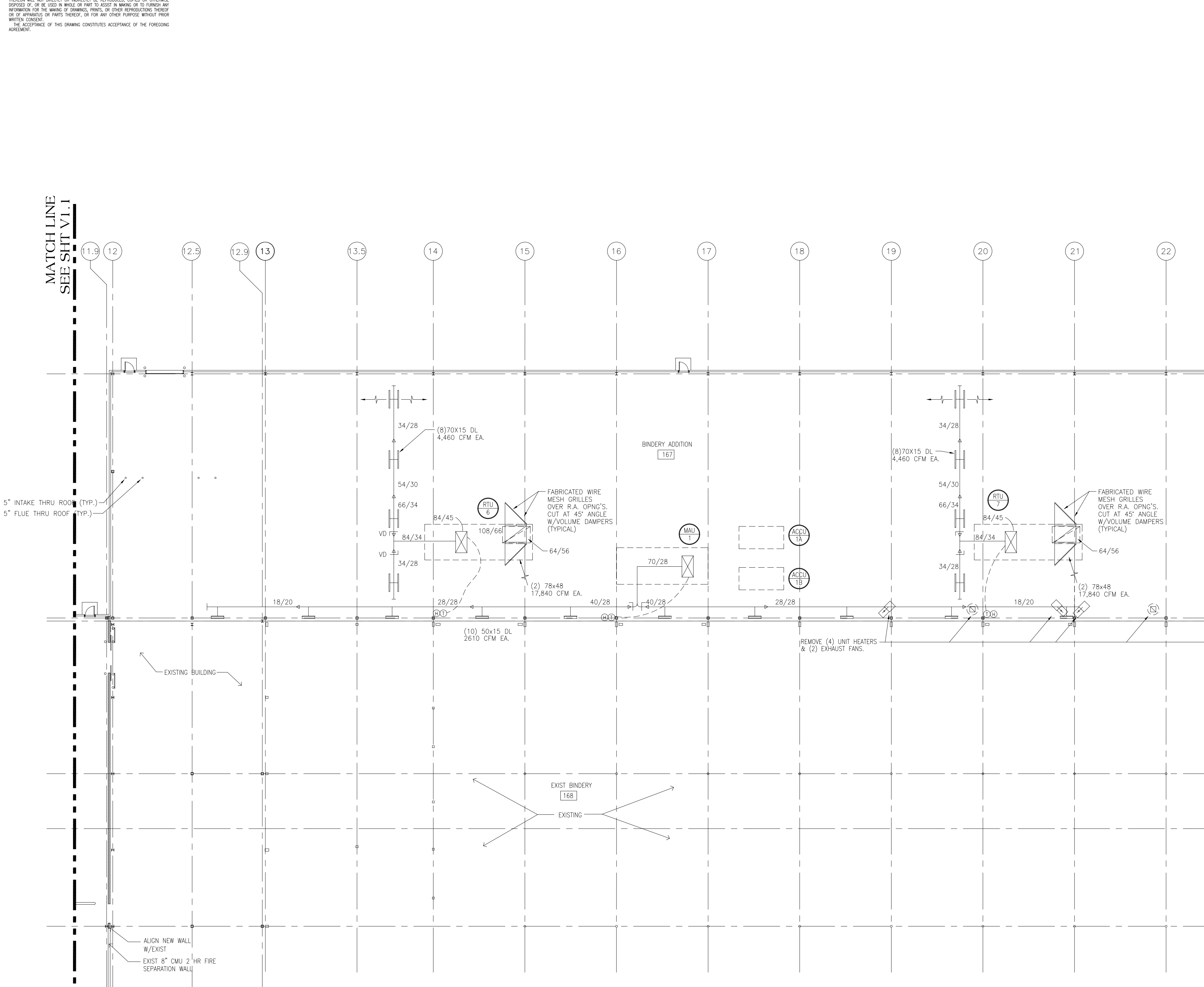
PARTIAL FLOOR PLAN-SOUTH SECTION SCALE: 1/16" = 1' - 0" NORTH
