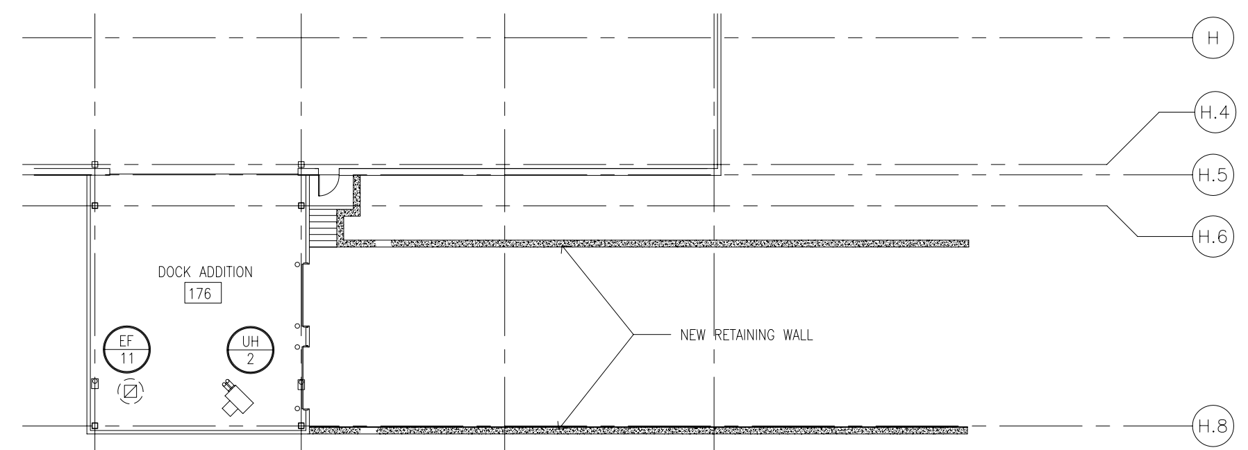
PARTIAL FLOOR PLAN OF DOCK ADDITION SCALE: 1/16" = 1' - 0" NORTH
