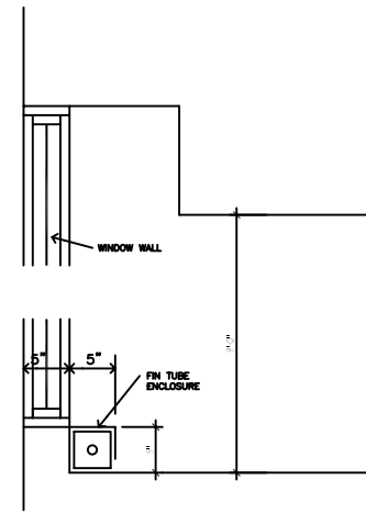
SECT THRU WINDOW WALL
