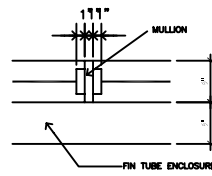
PLAN OF WINDOW WALL
