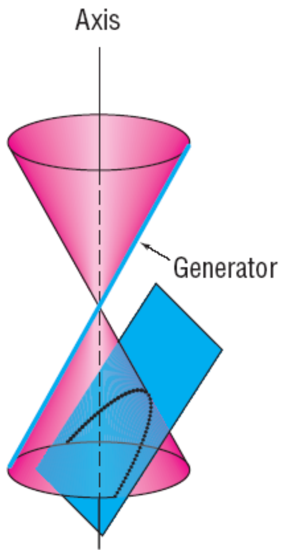
(c) Parabola
